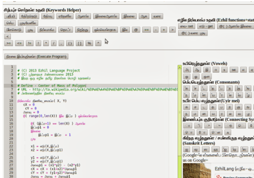
Figure 1: Ezhil online rich-text editor and evaluator http://ezhillang.org/koodam/play/eval/
